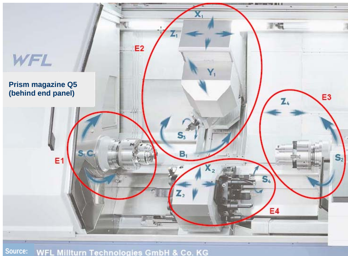
Figure 4: Different discrete hazards, with reference to the example of a machine tool
